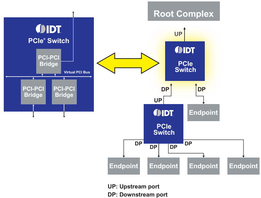
Figure 1. PCIe tree topology
