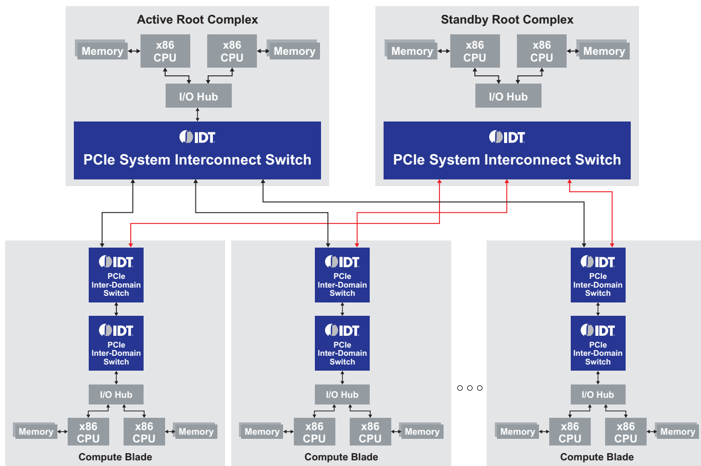
Figure 11. Dual-star redundancy
